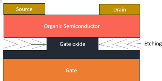
Fig.3 Dual cavity DM-OTFT structure
