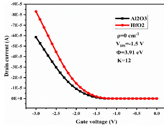
Fig.4 drain current analysis for Al 2 O 3 and HfO 2 .
