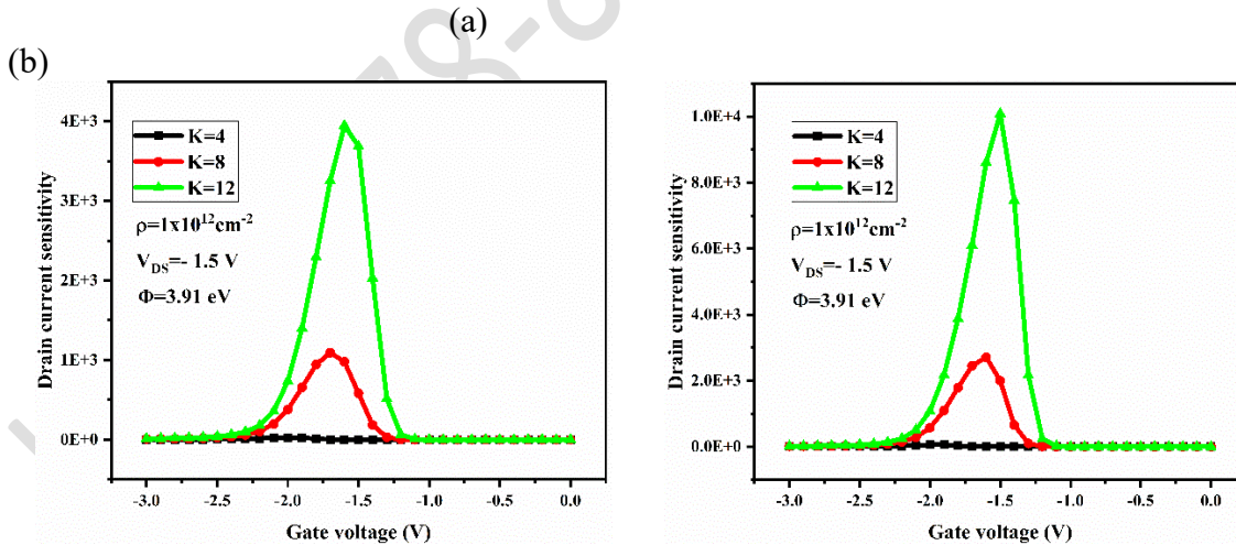
Fig. 5 Drain current sensitivity of charged biomolecule for a) Al 2 O 3 , b) HfO 2
